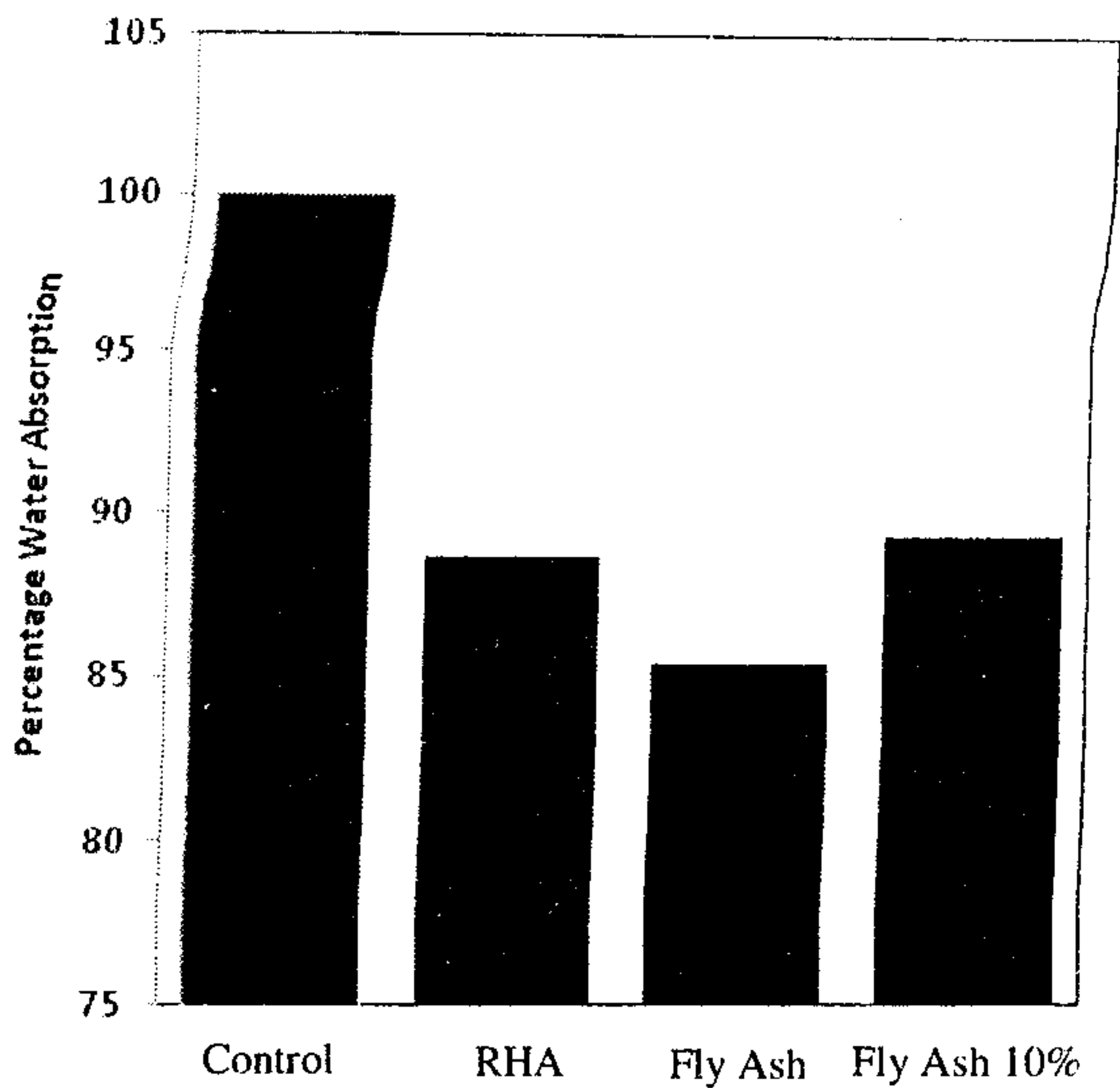
Figure 5: Surface water absorption test results
