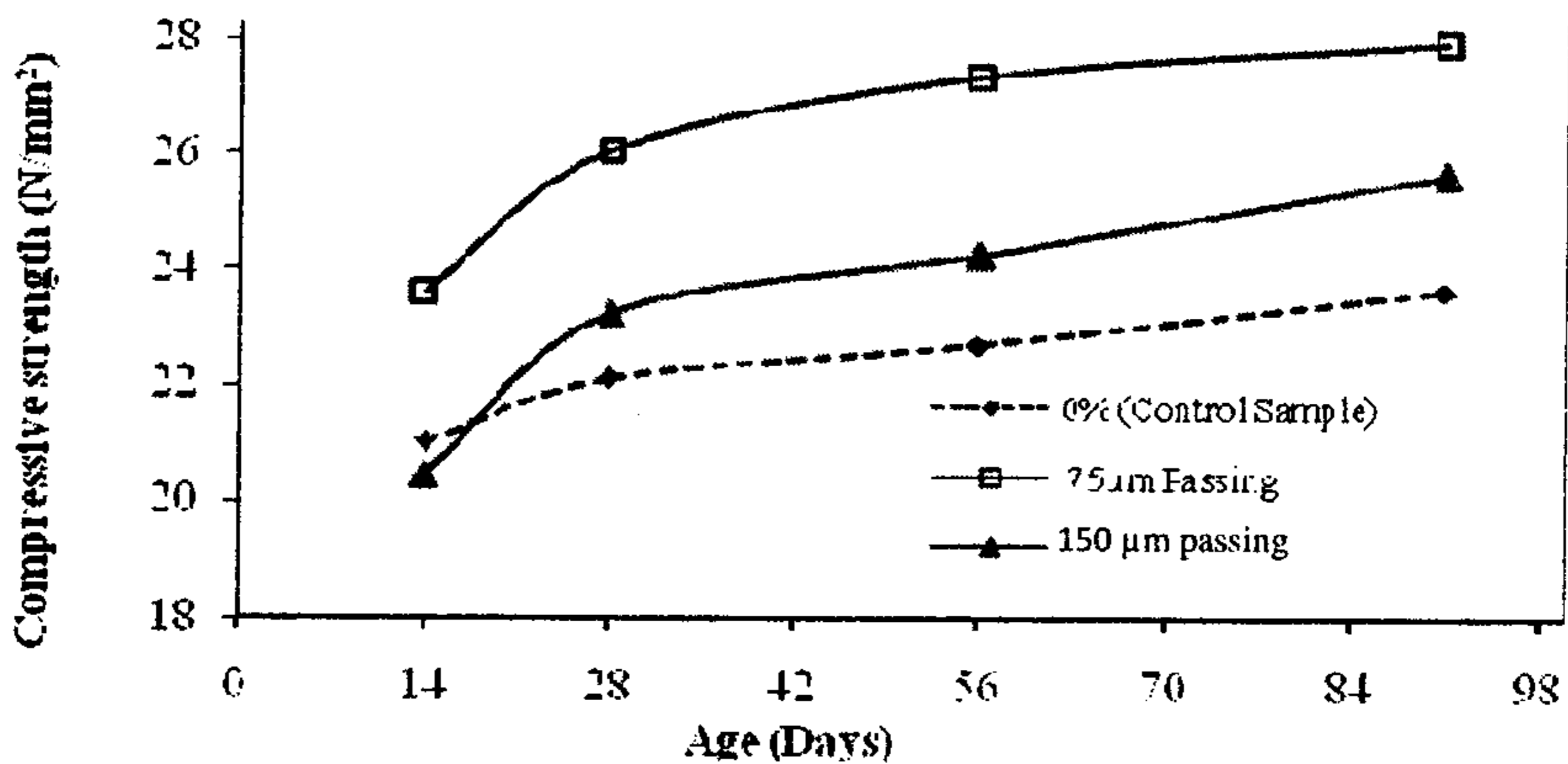
Figure 3: Variation of compressive strength of concrete with different sizes of particles of RHA
