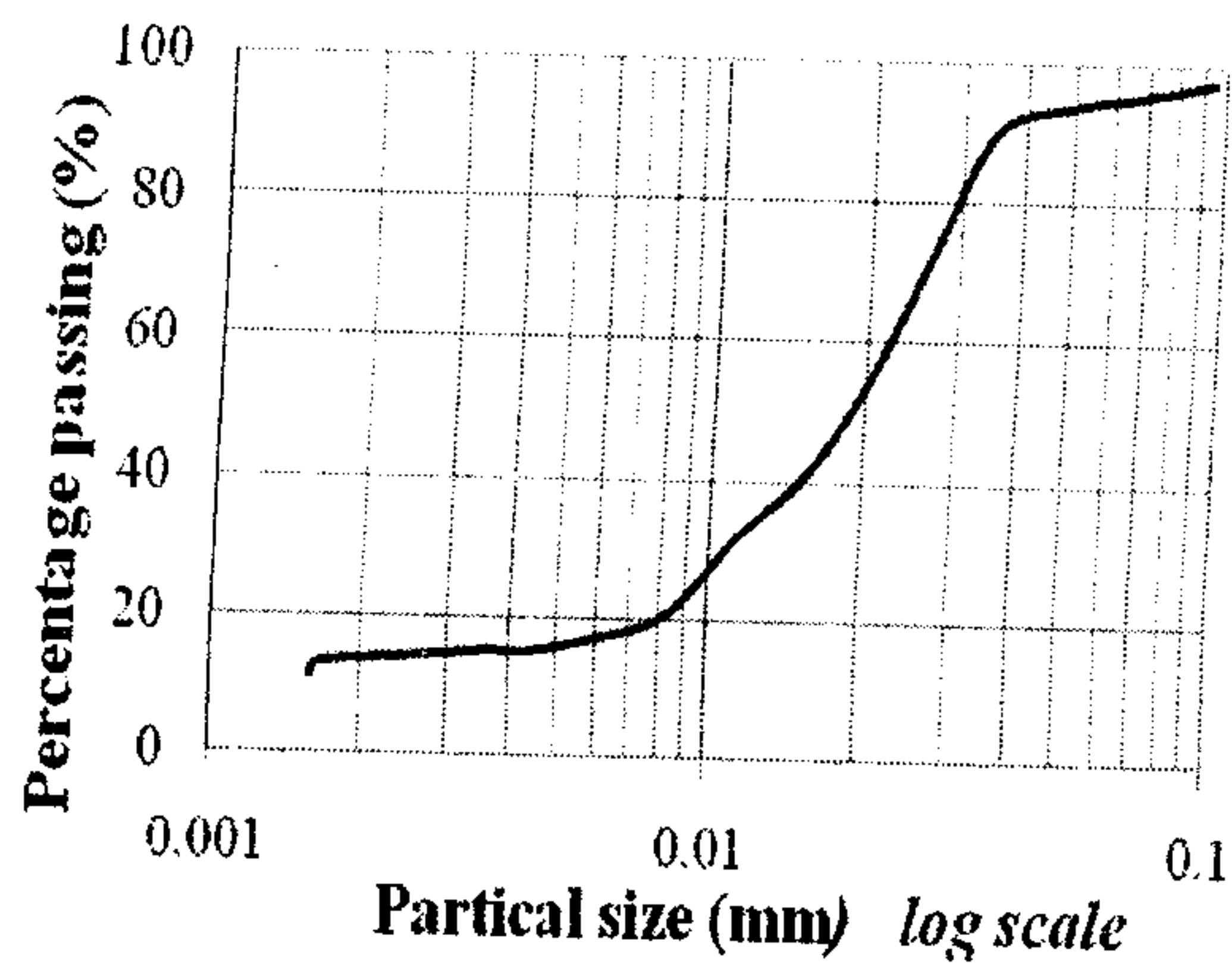
Figure 1: Particle size distribution for RHA obtained from 75µm passing
