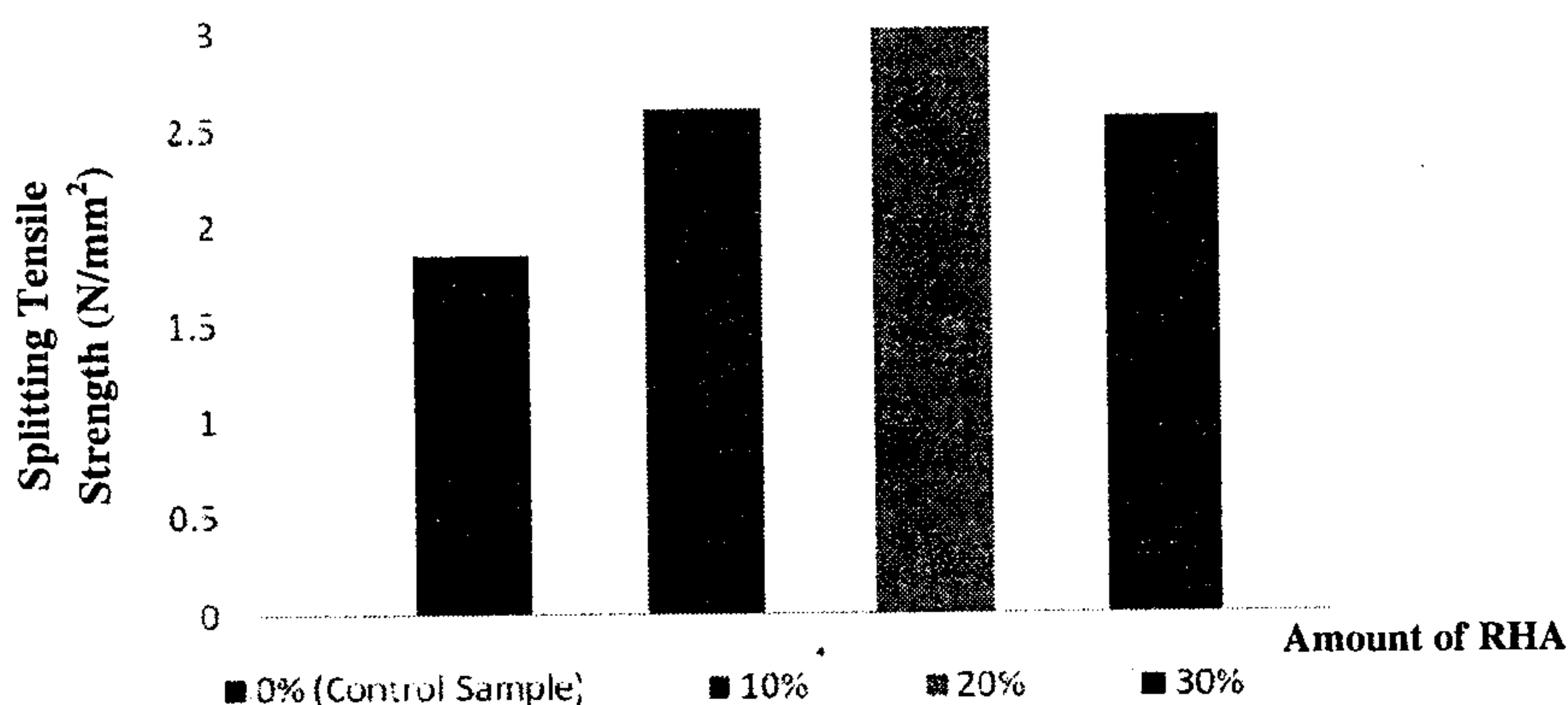
Figure 4: Variation of splitting tensile strength
