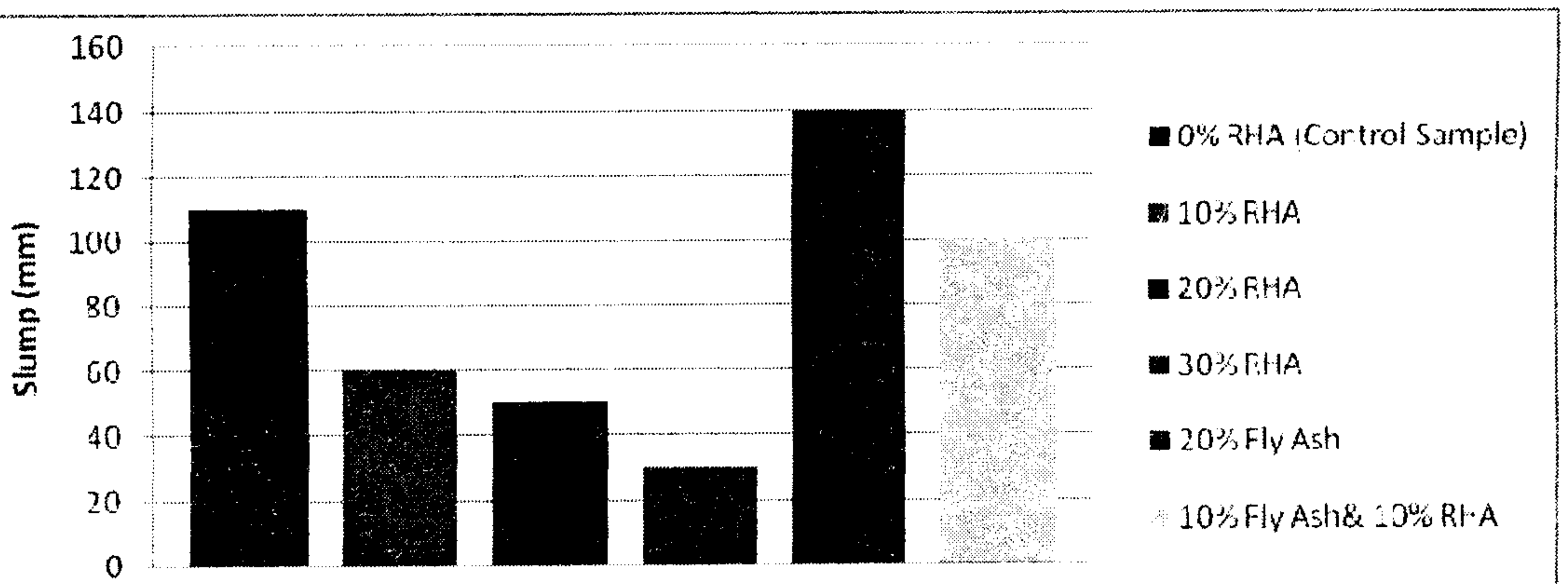
Figure 6: Variation of workability of concrete
