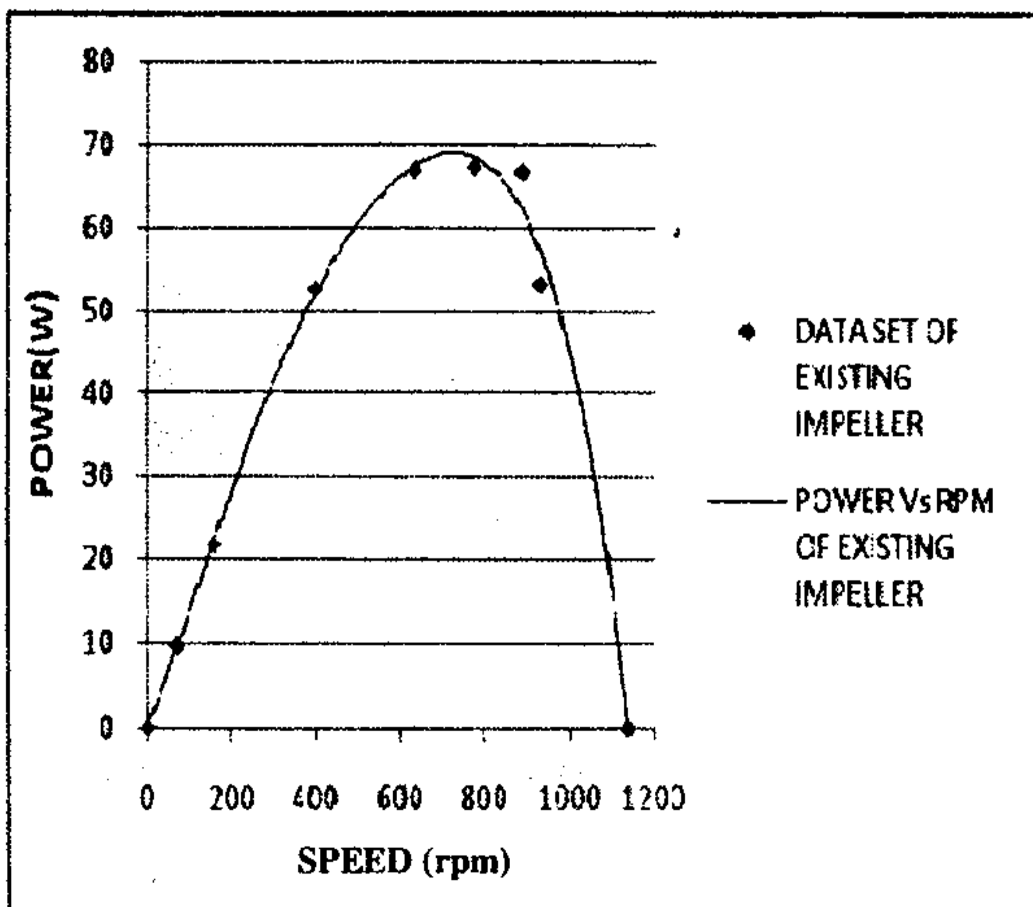
Graph 3.1: Power vs. rpm at Flow rate= 4.125 l/s
