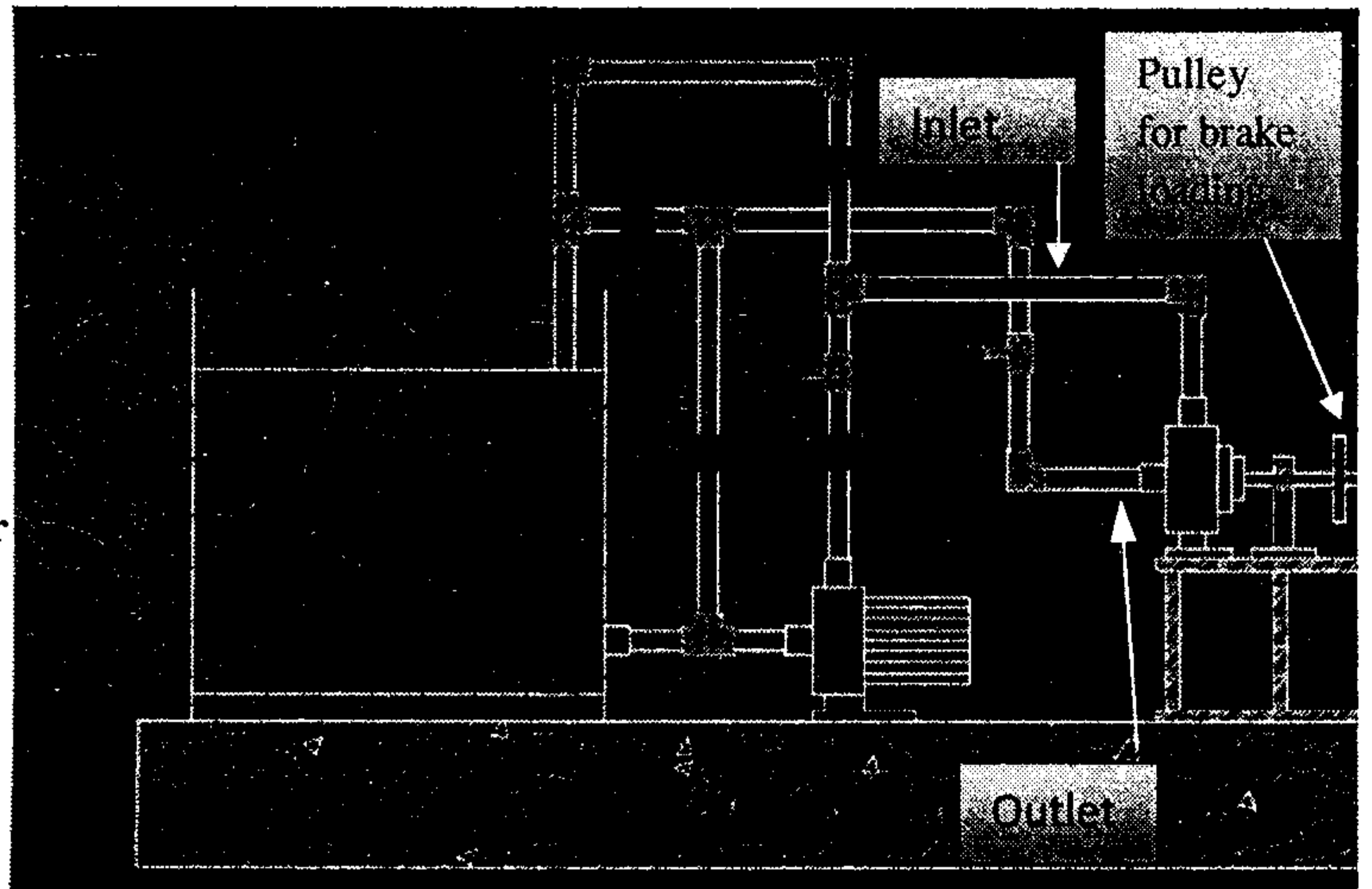
Fig. 3.16: Auto CAD Drawing of Test Bench for Brake Load Testing
