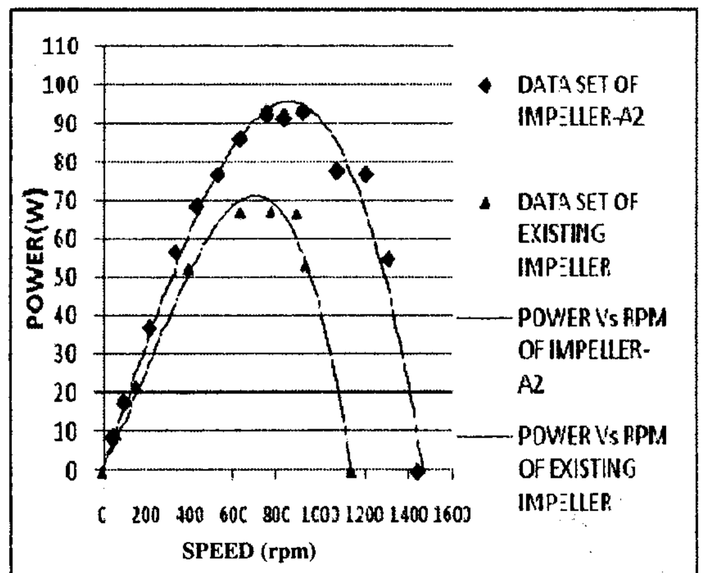
Graph 3.2: Power vs. rpm of Impeller-A2 and Existing Impeller
