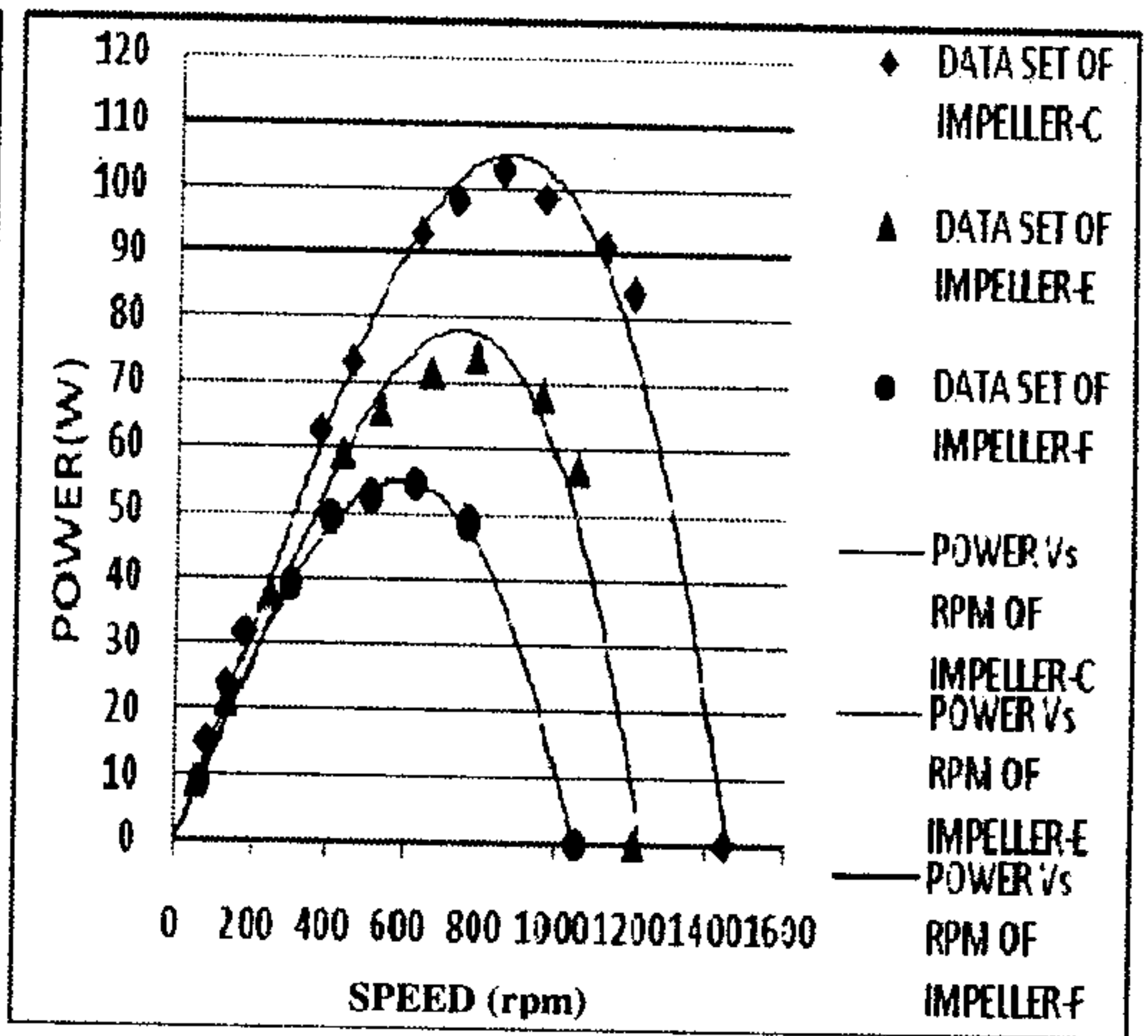
Graph 4.3: Power vs. rpm of Impeller-F, Impeller-E and Impeller-C
