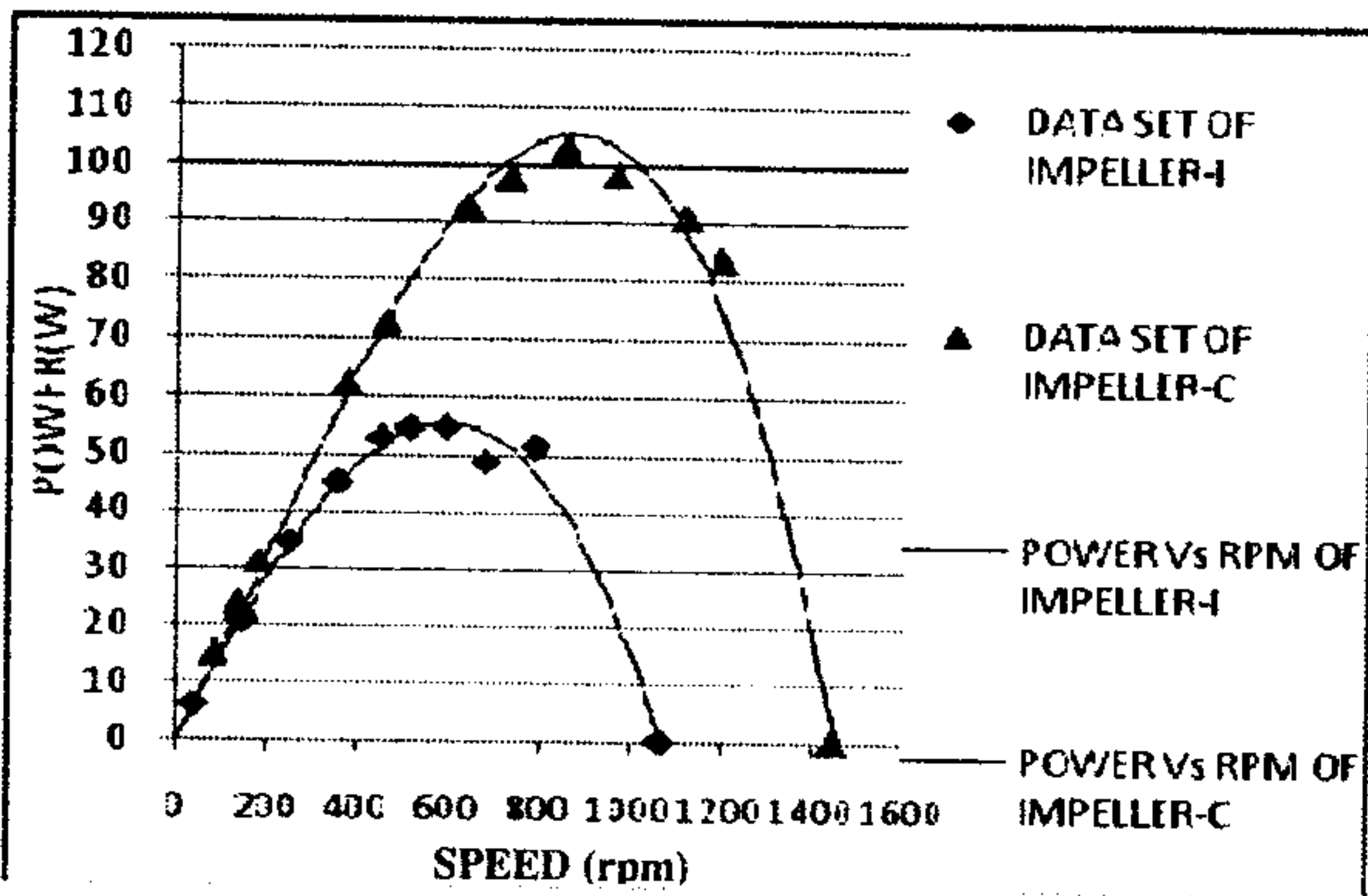
Graph 4.5: Power vs. rpm of Impeller-I and Impeller-C
