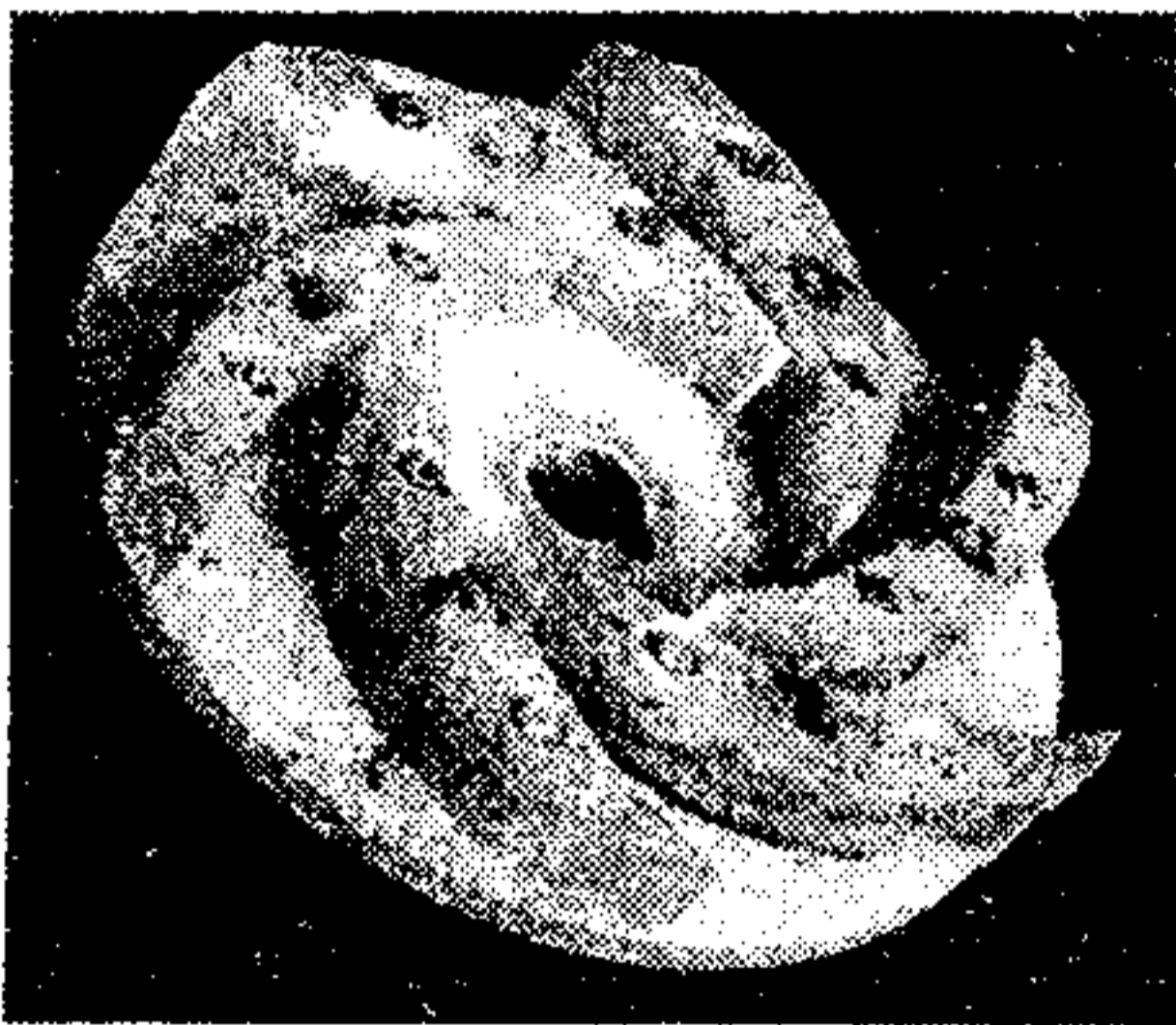
Fig. 3.15: Newly Designed Impeller
