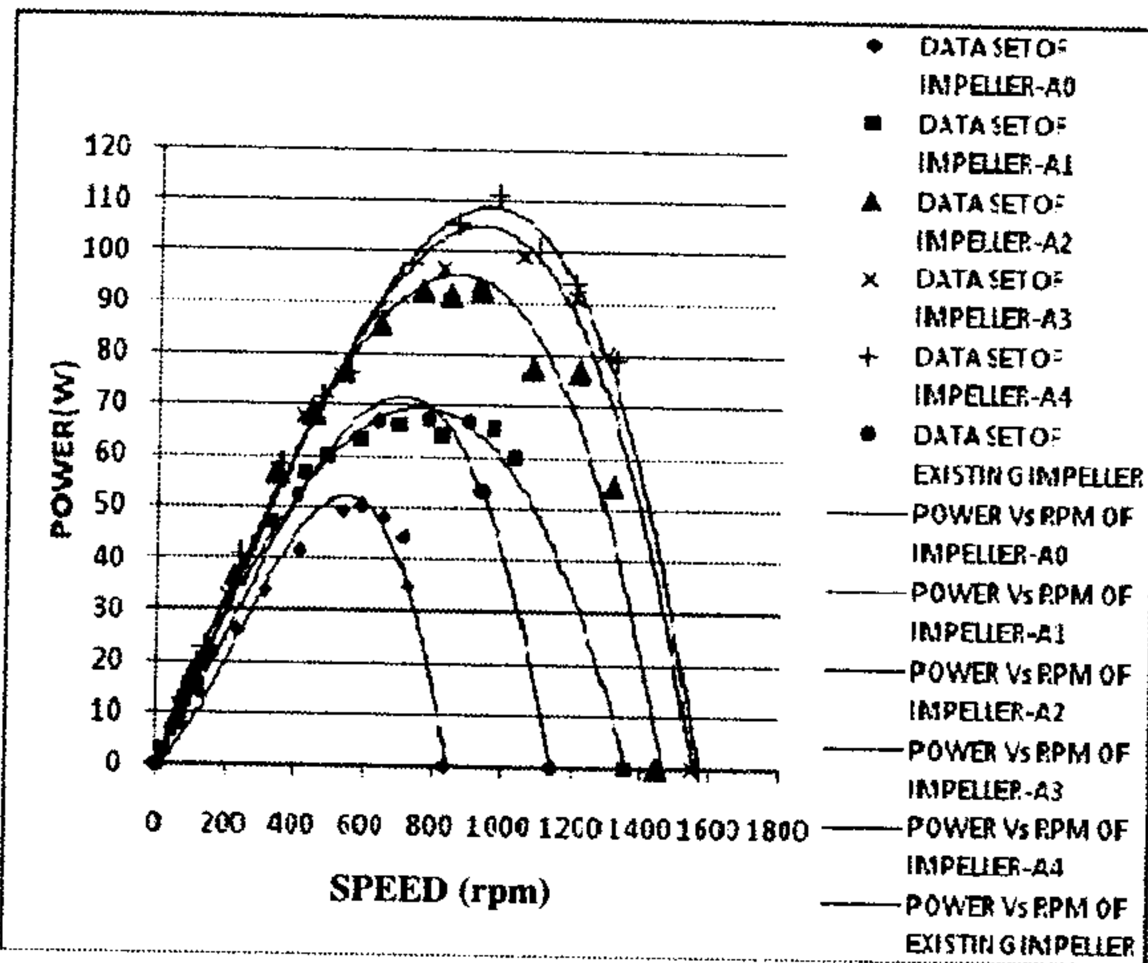
Graph 4.1: Power vs. rpm of Existing Impeller, Impeller-A, Impeller-A1, Impeller-A2, Impeller-A3 and impeller-A4
