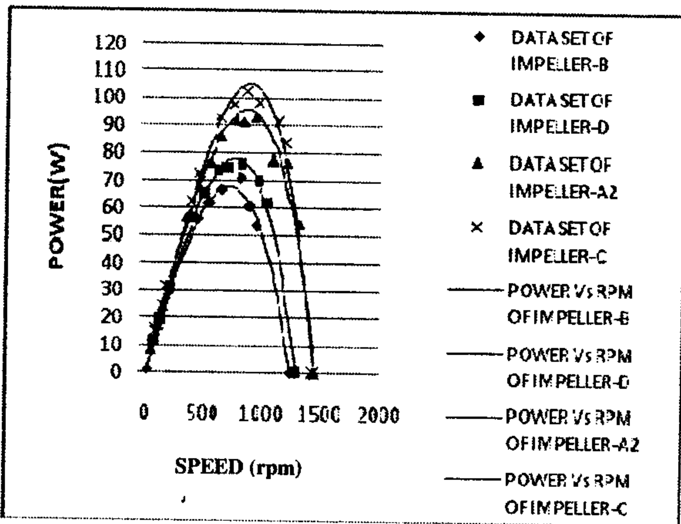
Graph 4.2: Power vs. rpm of Impeller-D, Impeller-B and Impeller-C
