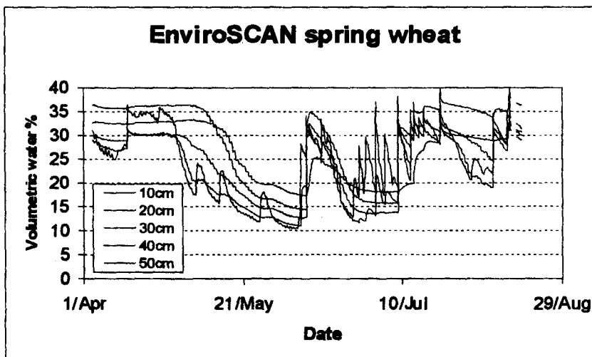
Fig. 4: Soil moisture measurement obtained using EnviroSCAN
