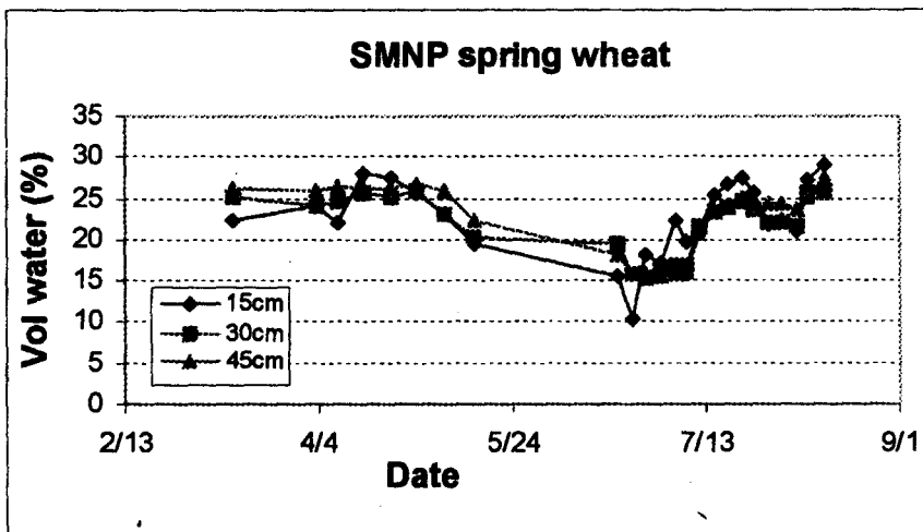
Fig. 3: Soil moisture measurement obtained using neutron probe
